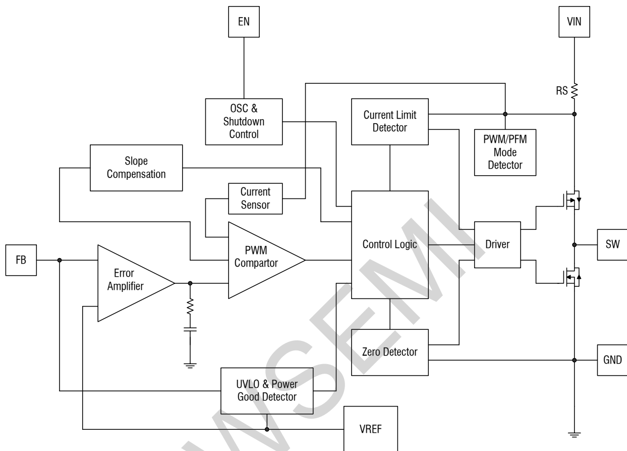
Figure 2. HX3406 Block Diagram
