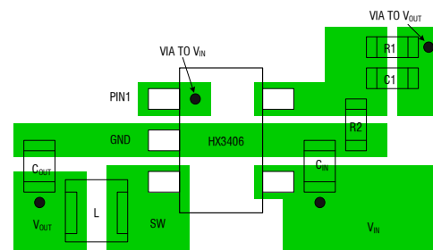
Figure 3. HX3406 Suggested Layout
