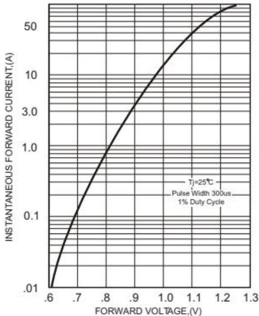
FIG.1-TYPICAL FORWARD CHARACTERISTICS
