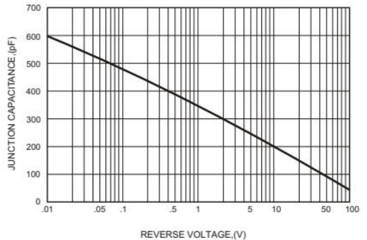
FIG.5-TYPICAL JUNCTION CAPACITANCE
