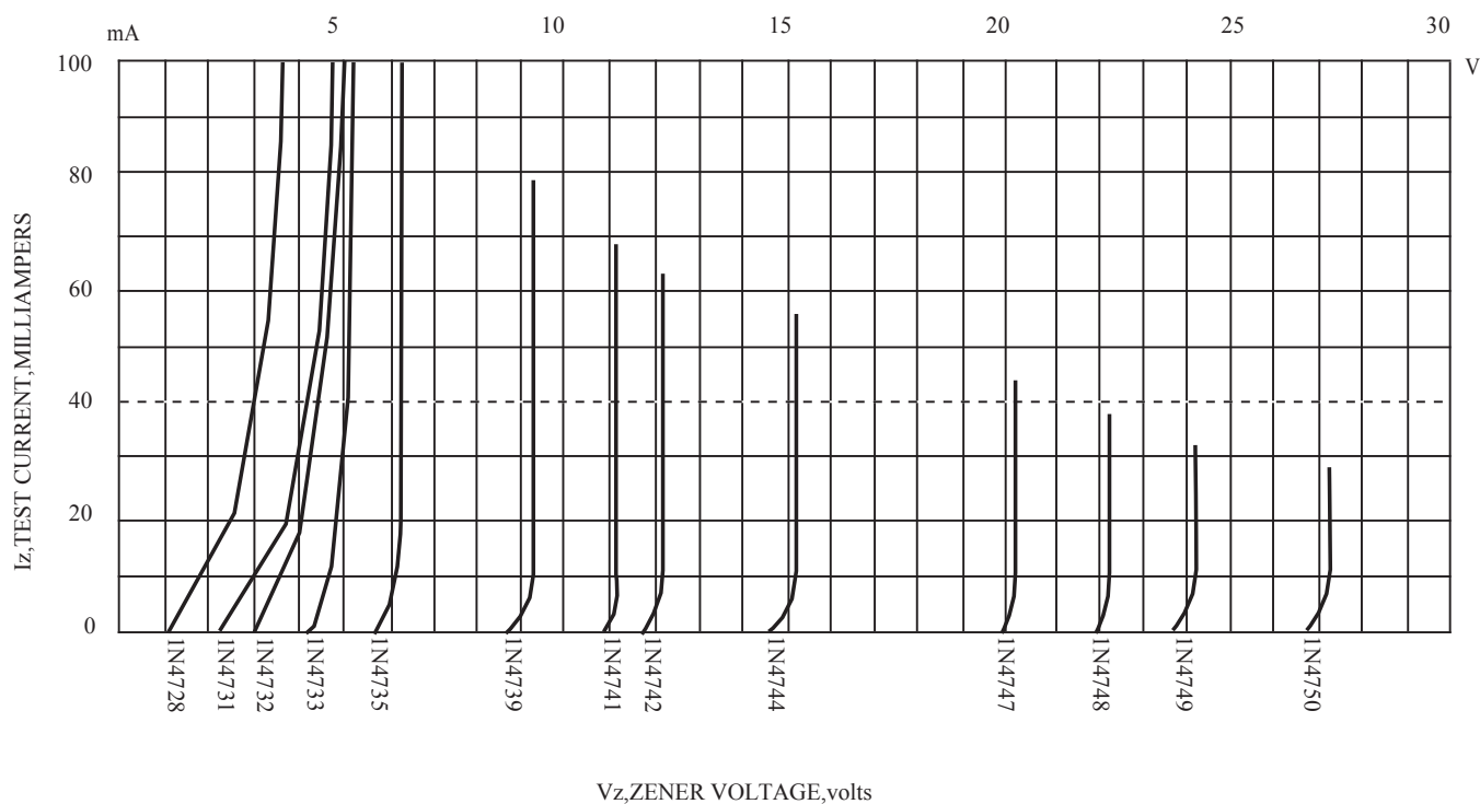
Breakdown characteristics
