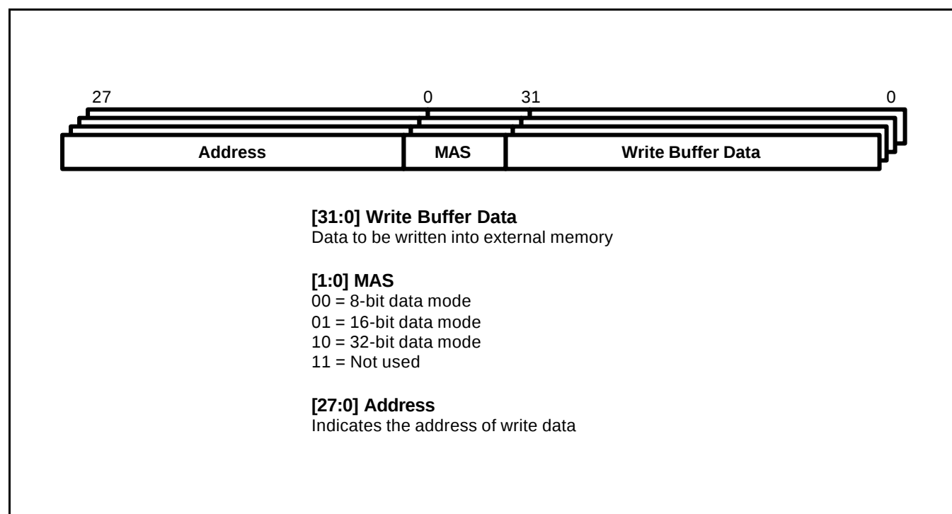
Figure 6-4. Write Buffer Configuration
