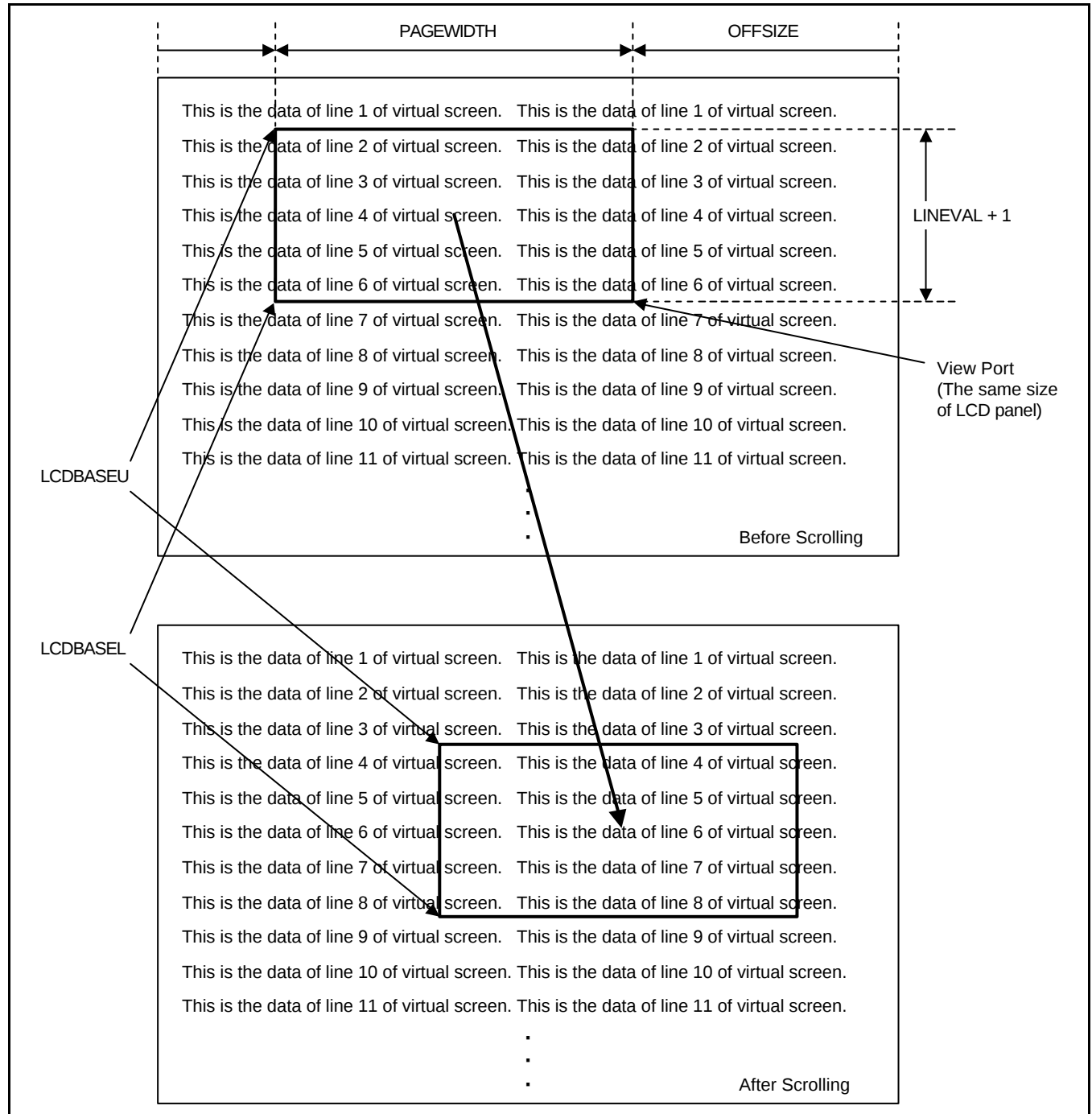
Figure 12-6. Example of Scrolling in Virtual Display(single scan)
