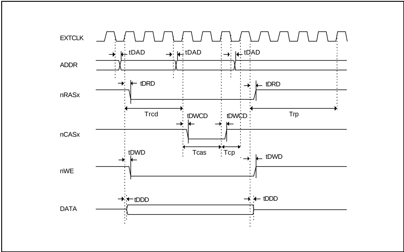
Figure 19-25. DRAM(FP/EDO) Single Write Timing ( T_{rcd}=3 , T_{cas}=2 , T_{cp}=1 , T_{rp}=4.5 , MT=01/10b )
