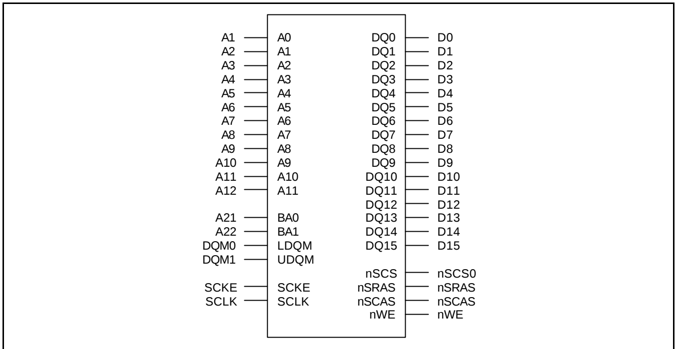
Figure 4-10. Memory Interface with 16bit SDRAM (4Mx16, 4bank)
