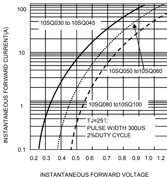
FIG.4-TYPICAL FORWARD CHARACTERISTICS
