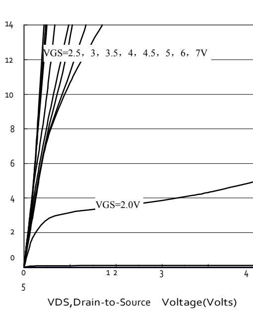
Figure 1. Output Characteristics
