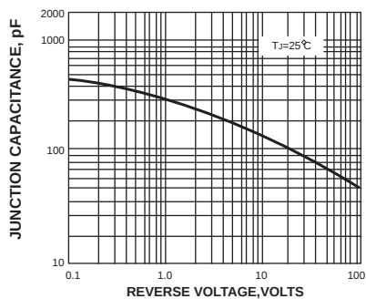
FIG. 5-TYPICAL JUNCTION CAPACITANCE
