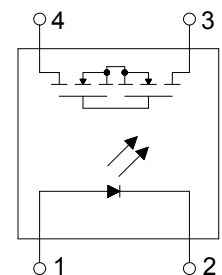
1 FORM A NORMALLY OPEN
