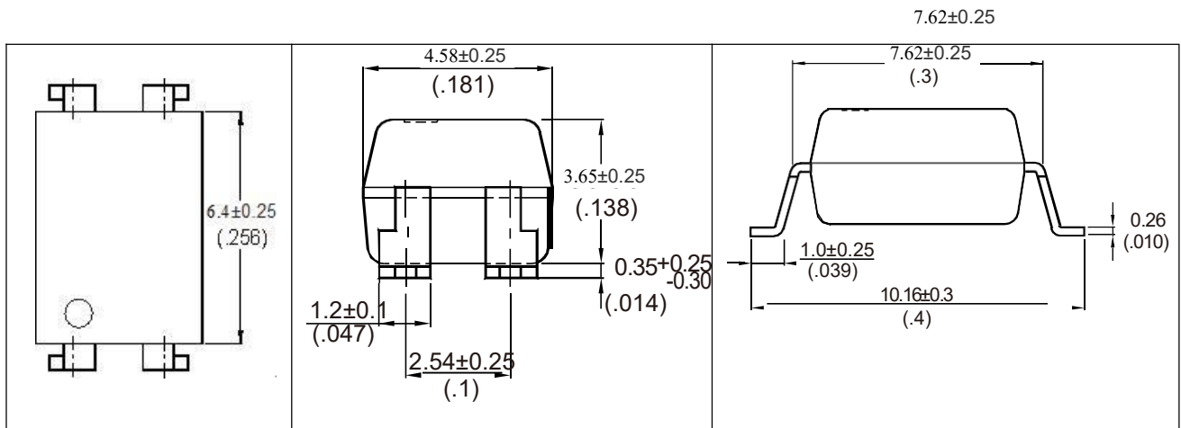
4-pin SMD
