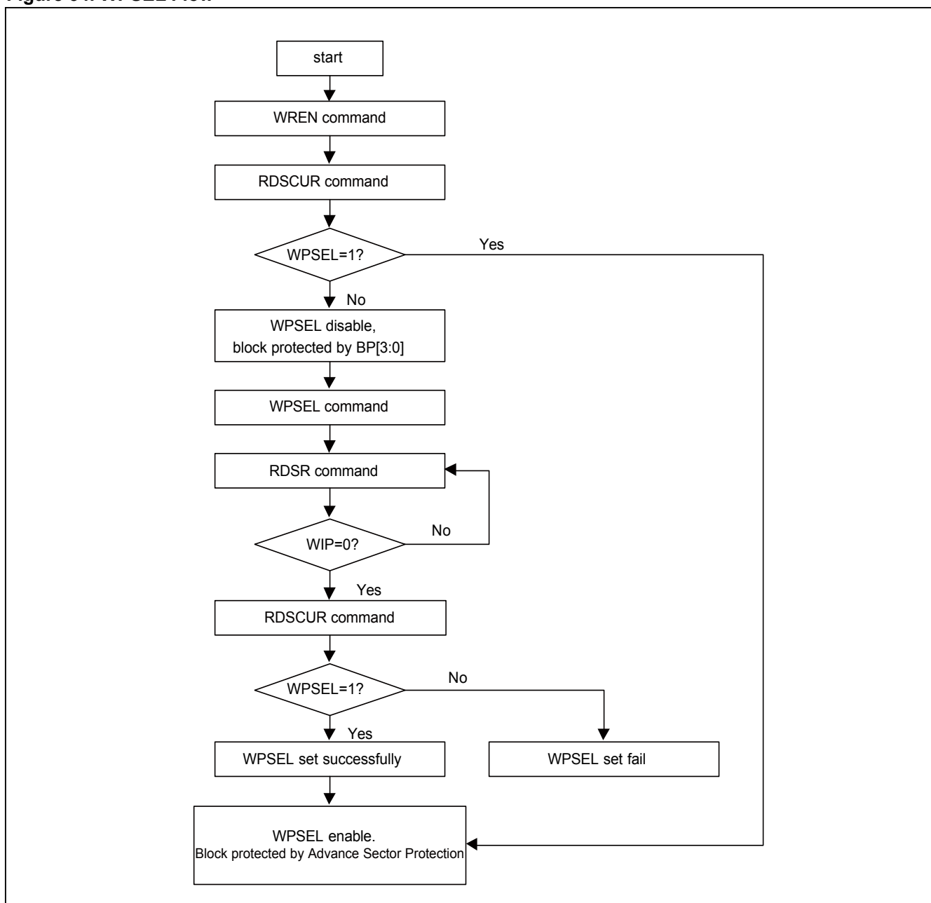
Figure 34. WPSEL Flow
