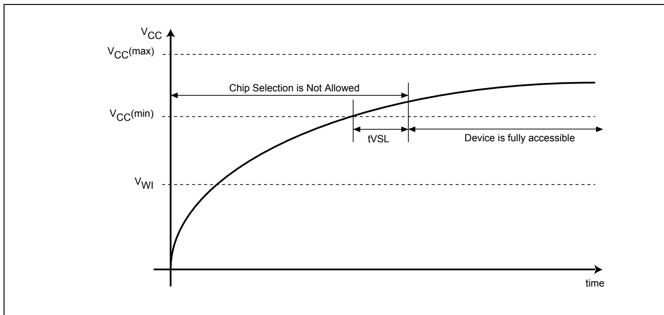
Figure 57. Power-up Timing
