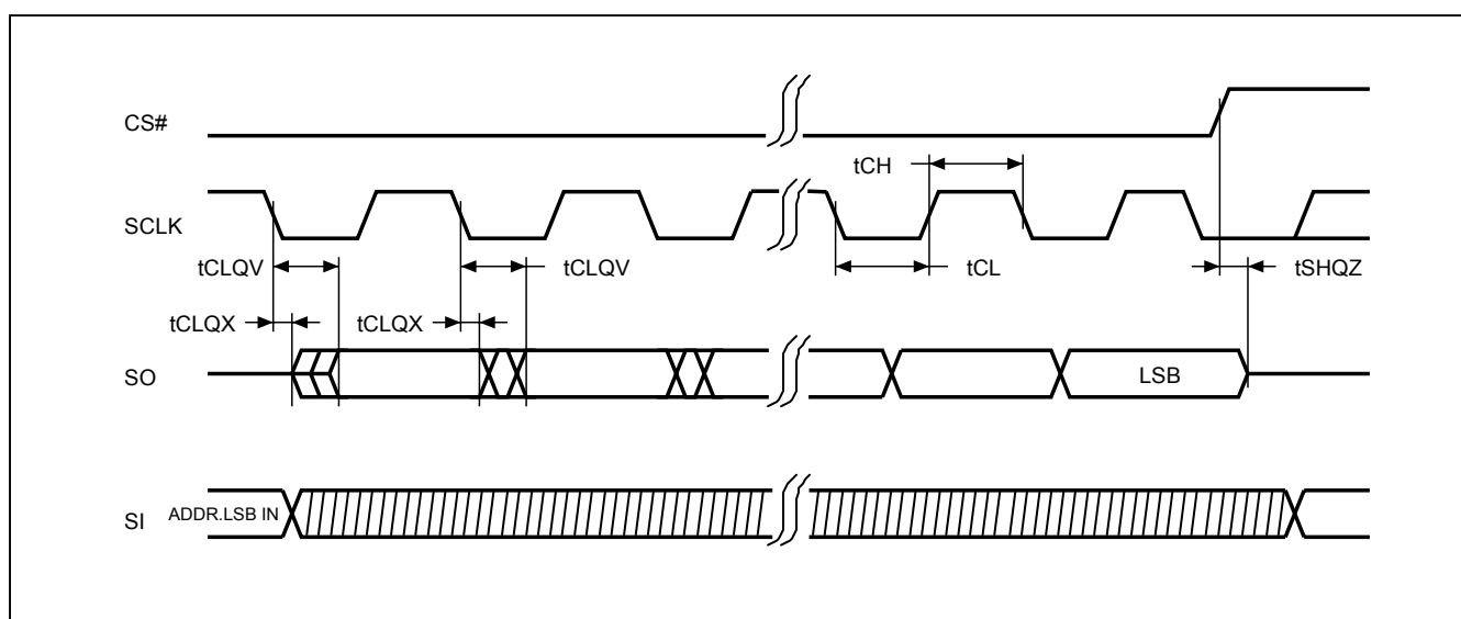
Figure 52. Output Timing
