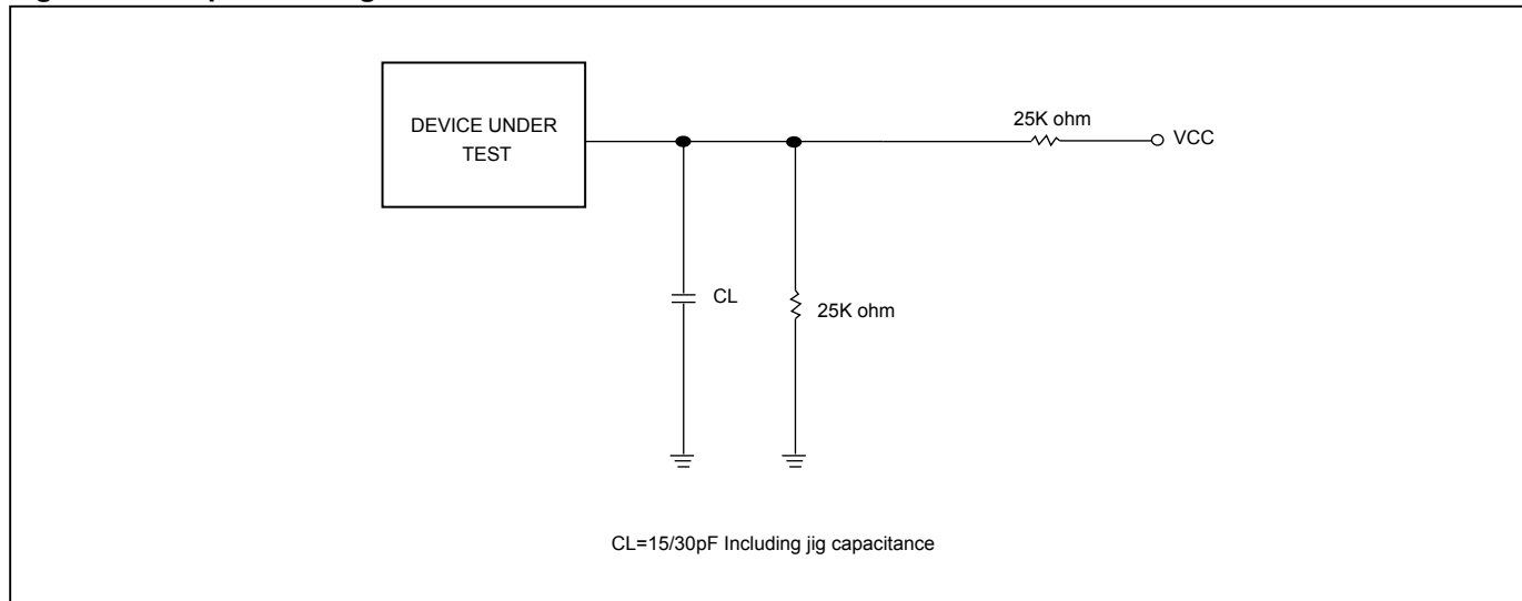
Figure 36. Output Loading
