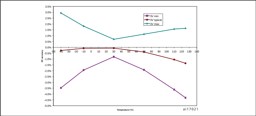
Figure 17. Typical HSI accuracy at V_{DD} = 3\text{ V} vs temperature
