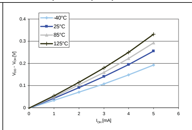
Figure 29. Typ. V_{DD} - V_{OH} @ V_{DD} = 1.8 V (standard ports)
