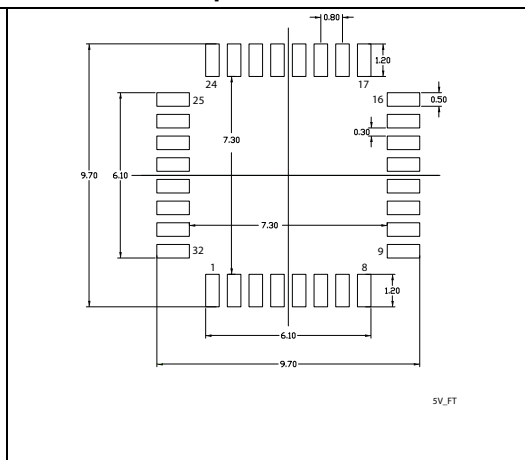
Figure 40. LQFP32 recommended footprint (1)(2)
