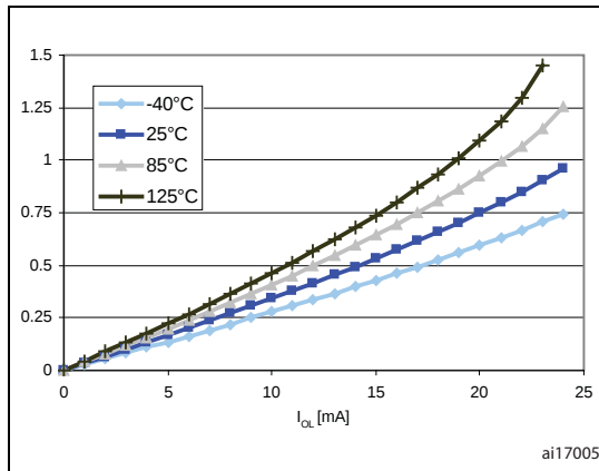
Figure 24. Typ. V_{OL} @ V_{DD} = 3.0 V (standard ports)
