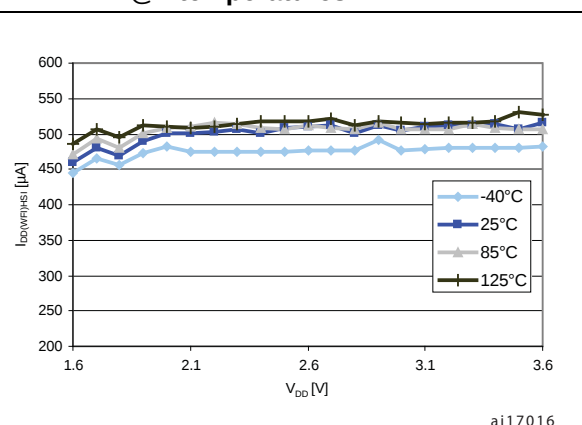
Figure 14. I_{DD(WAIT)} vs. V_{DD} @ f_{CPU} = 16\text{ MHz} @4 temperatures
