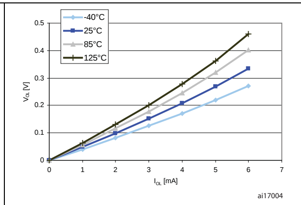
Figure 25. Typ. V_{OL} @ V_{DD} = 1.8 V (standard ports)
