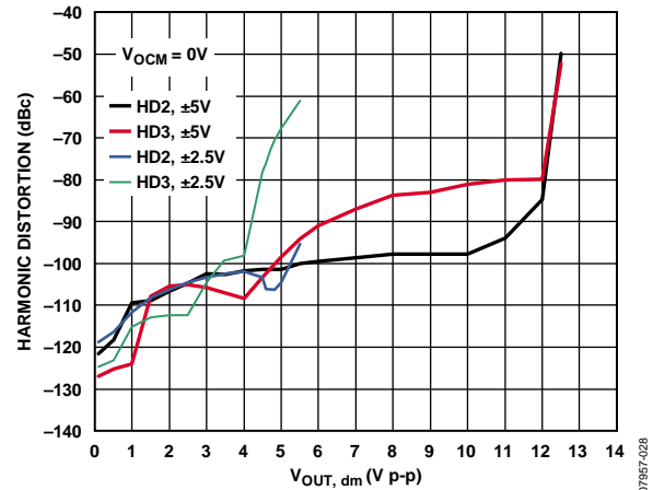
Figure 28. Harmonic Distortion vs. V_{OUT, dmV} f = 10 MHz
