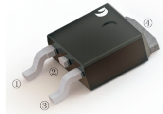
TO-252(D-PAK)
