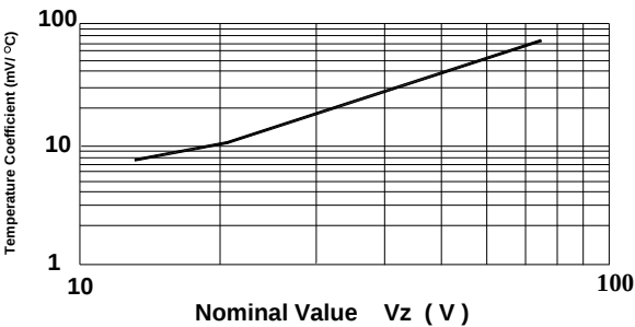
Temperature Coefficient
