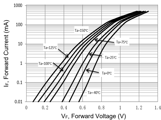
Fig 4. Forward Characteristics
