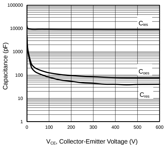
Figure 5 Capacitance Characteristics
