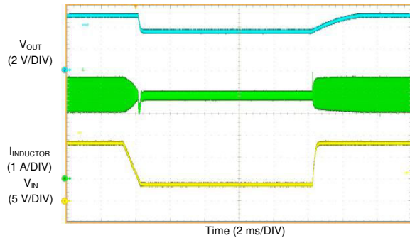
图 10-35. LM61460-Q1 Short Circuit Recovery
