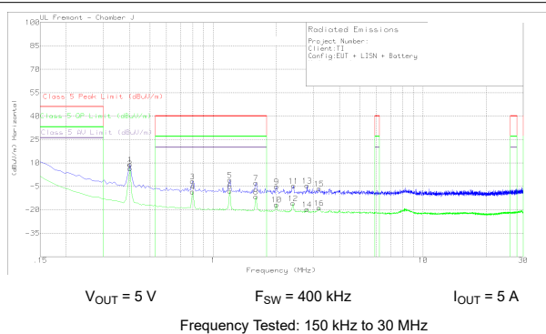
图 10-48. Radiated EMI Rod versus CISPR25 Limits
