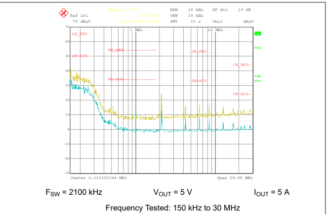
图 10-54. Conducted EMI versus CISPR25 Limits (Yellow: Peak Signal, Blue: Average Signal)
