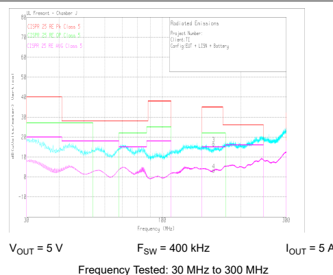
图 10-50. Radiated EMI Bicon Horizontal versus CISPR25 Limits
