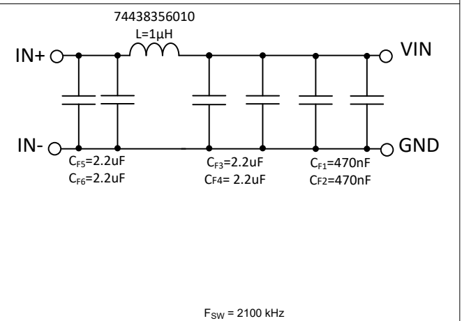
图 10-56. Recommended Input EMI Filter
