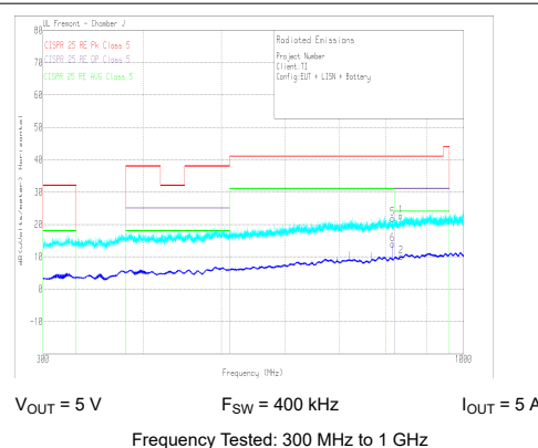
图 10-52. Radiated EMI Log Horizontal versus CISPR25 Limits
