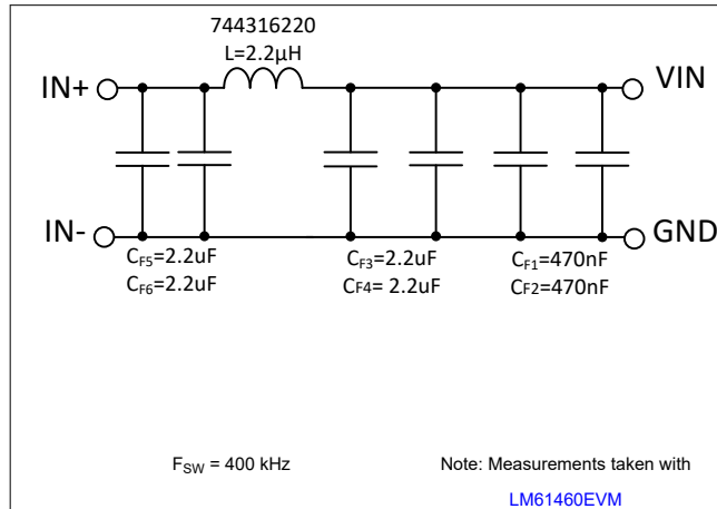
图 10-53. Recommended Input EMI Filter
