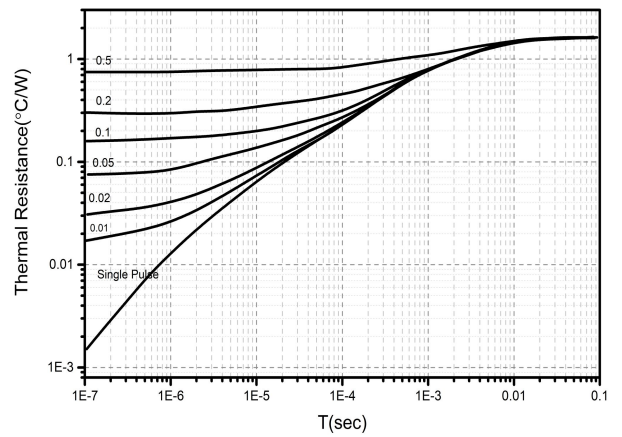
Figure 10. Transient Thermal Impedance (TO-251 TO-252)
