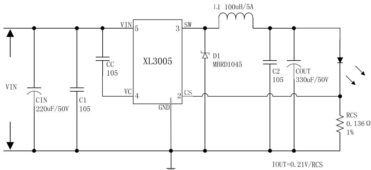
Figure19. XL3005 System Parameters Test Circuit (VIN=8V~36V, IOU=1540mA)
