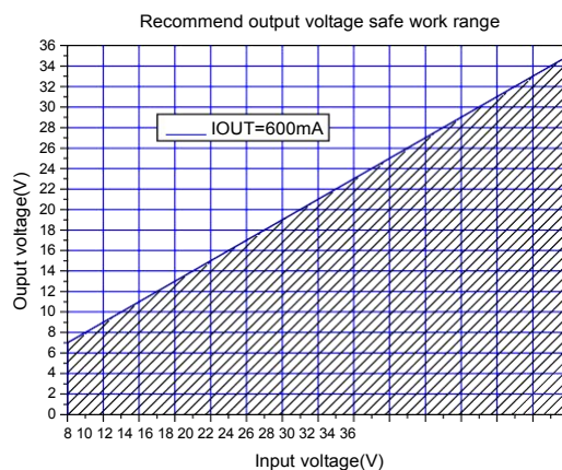
Figure6.Max output voltage(IOUT=600mA)
