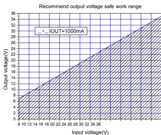
Figure7.Max output voltage(IOUT=1000mA)
