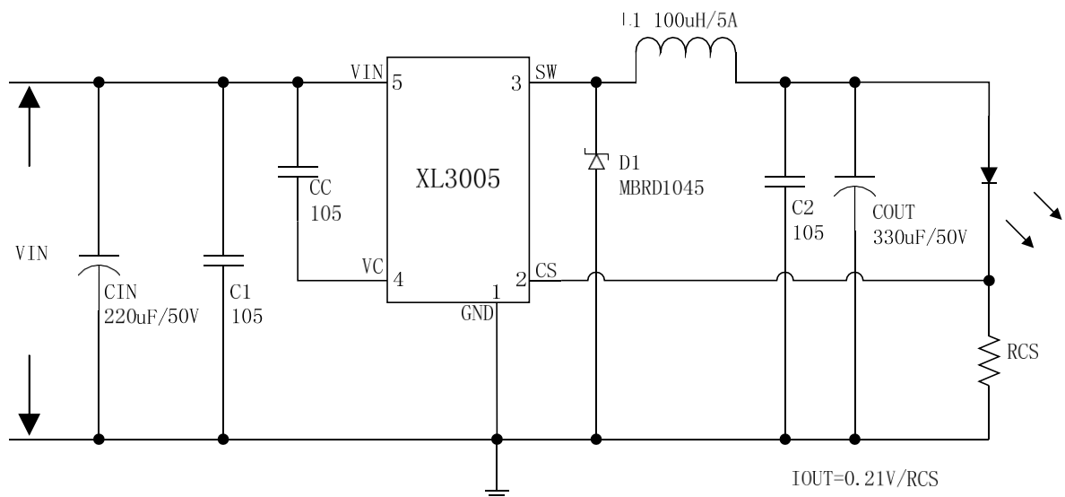
Figure4. XL3005 Typical Application Circuit
