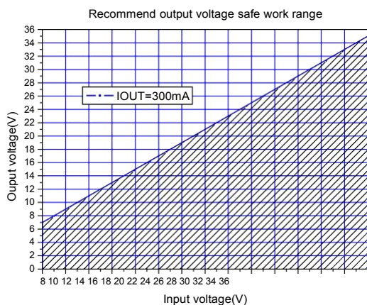
Figure5.Max output voltage(IOUT=300mA)
