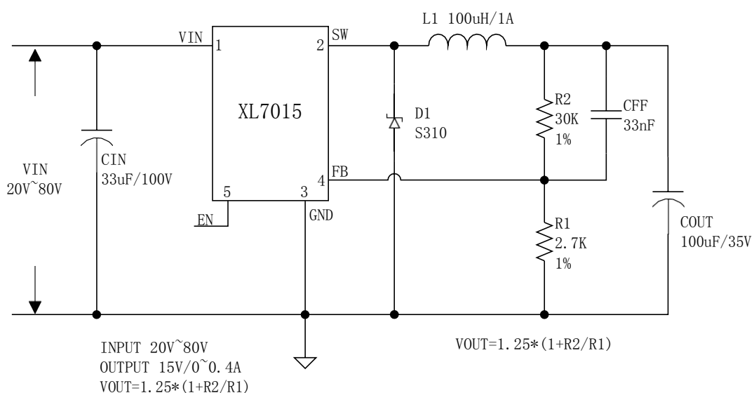
Figure4. XL7015 Typical Application Circuit
