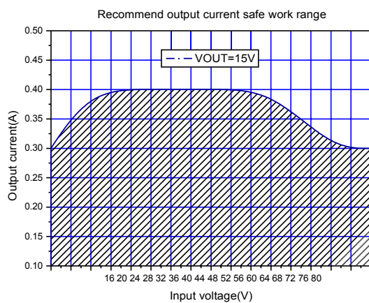
Figure7.Max output current(VOUT=15V)
