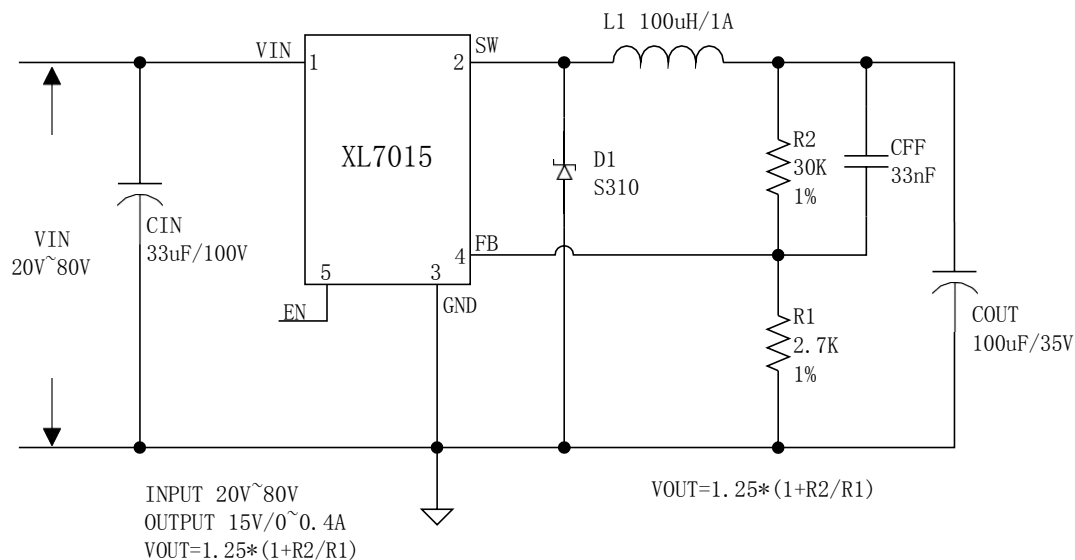
Figure8. XL7015 System Application (VIN=20V~80V, VOUT=15V/0.4A)
