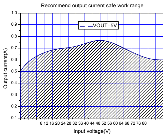
Figure5.Max output current(VOUT=5V)
