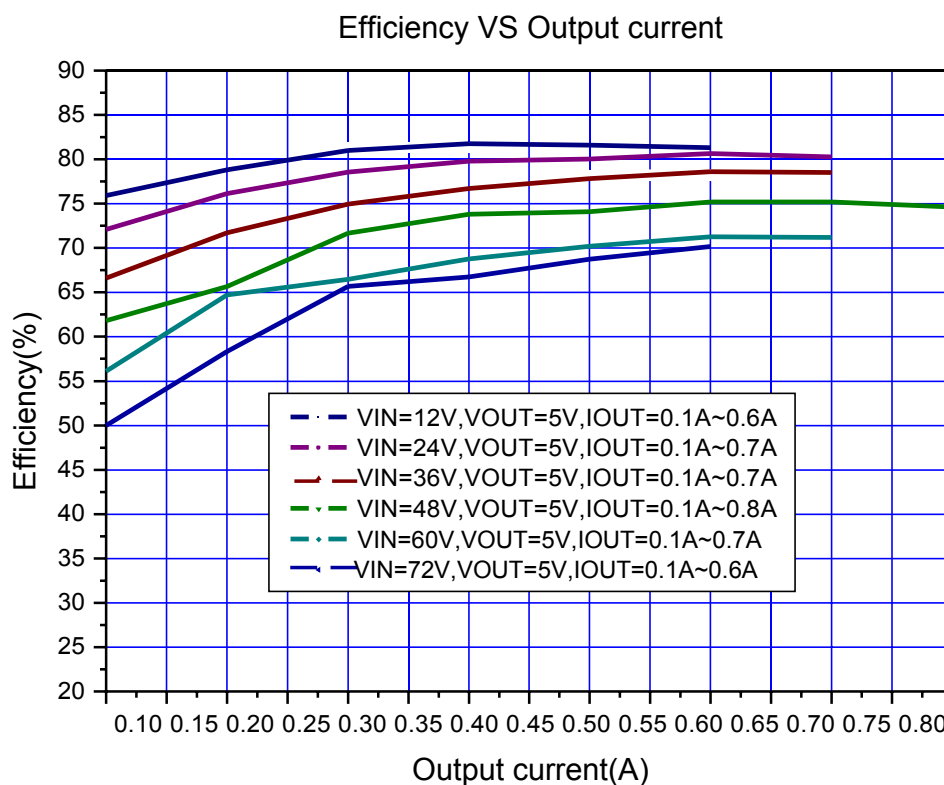
Figure11. XL7015 System Application (Efficiency VS Output Current)
