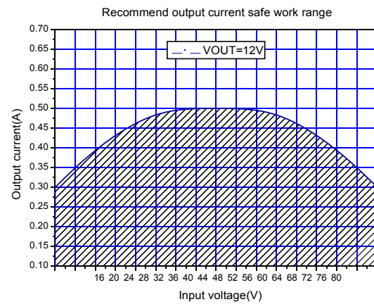
Figure6.Max output current(VOUT=12V)
