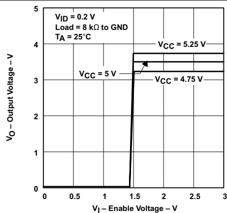
图 6-8. Receiver Output Voltage vs Enable Voltage
