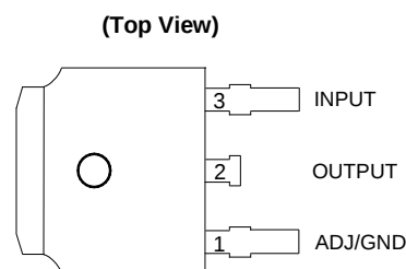
TO252-2 (3) Option 2
