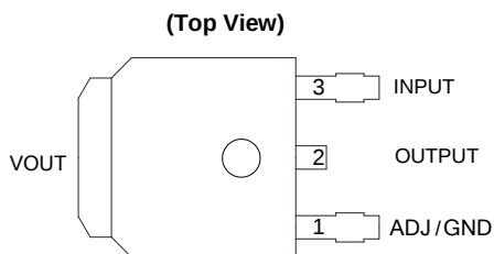
TO252-2 (4)
