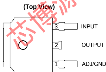
TO252-2 (3) Option 1
