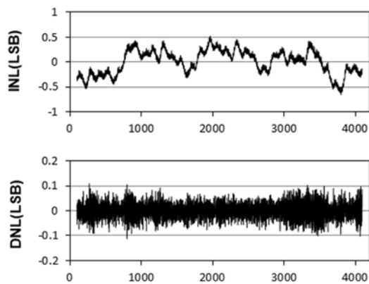
INL and DNL vs. Digital Input Code ( -40^\circ C TPC112S1)
