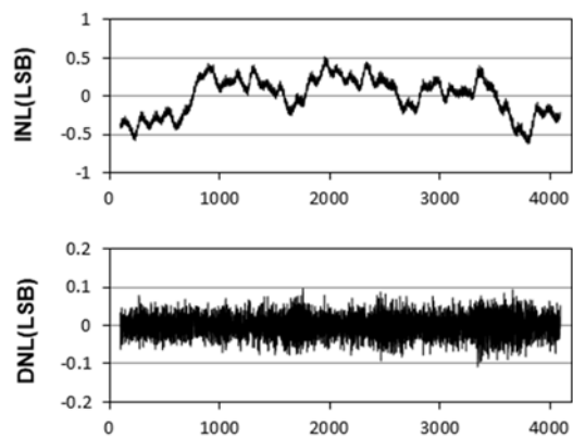
INL and DNL vs. Digital Input Code ( 25^\circ C TPC112S1)
