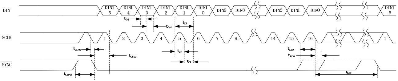
Figure 1. 16-Bit Serial-Interface Timing Diagram (TPC112S1)
