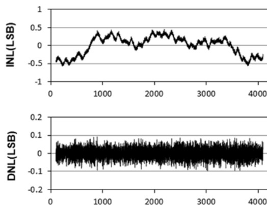
INL and DNL vs. Digital Input Code ( 125^\circ C TPC112S1)
