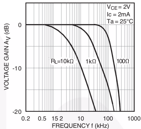
Fig. 14 Frequency Response
