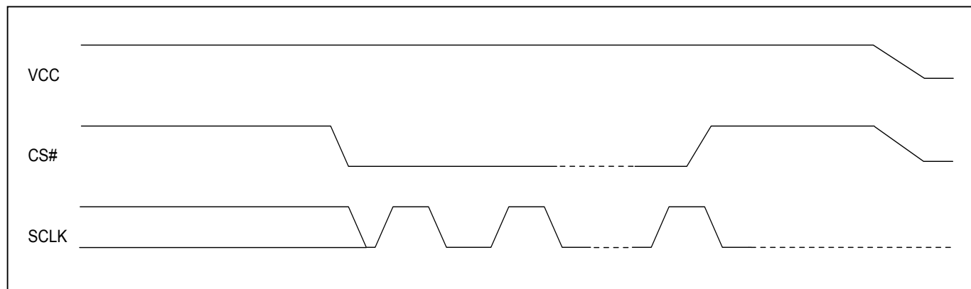
Figure 29. Power-Down Sequence
