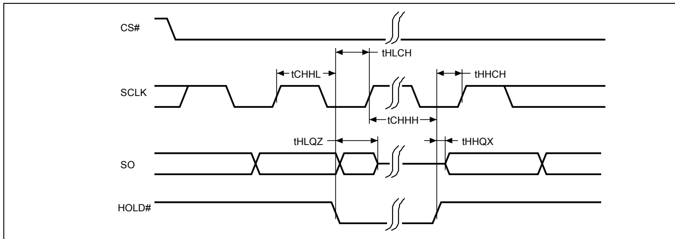
Figure 9. Hold Timing
