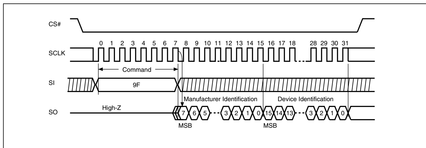
Figure 13. Read Identification (RDID) Sequence (Command 9F)
