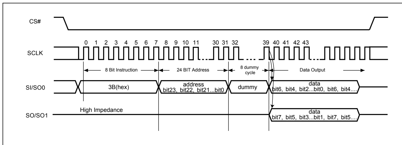
Figure 18. Dual Output Read Mode Sequence (Command 3B)
