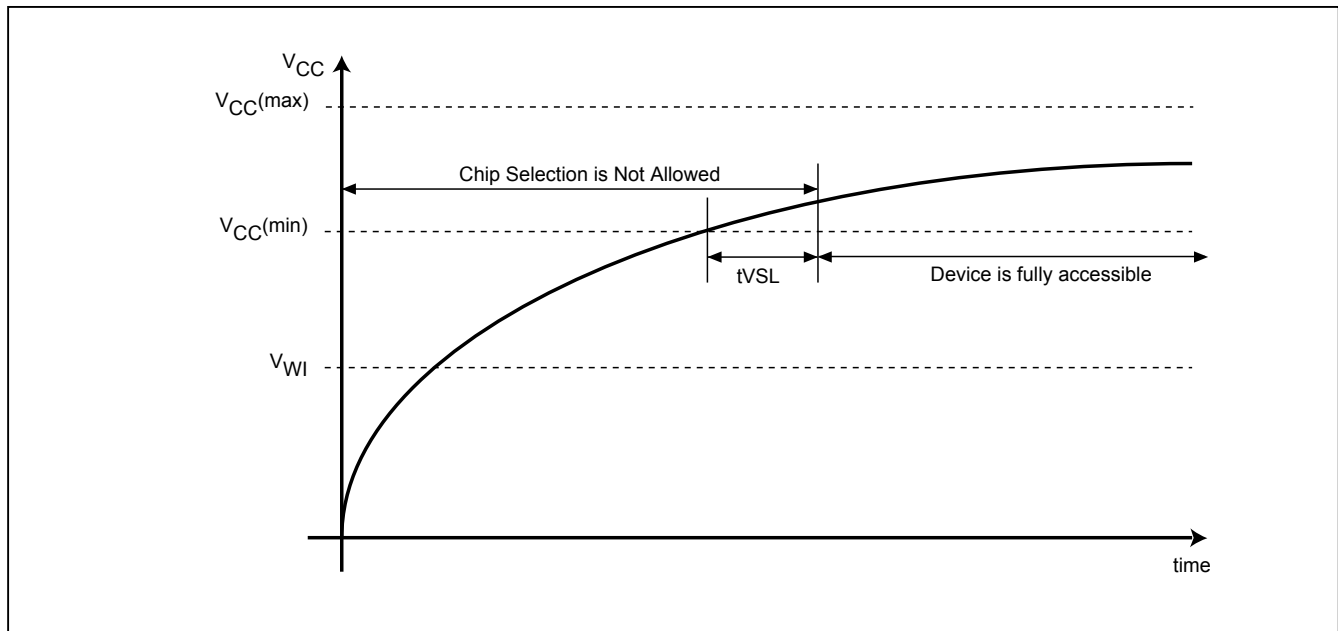
Figure 48. Power-up Timing
