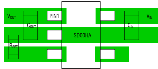
Figure 3. SD00HA Suggested Layout
