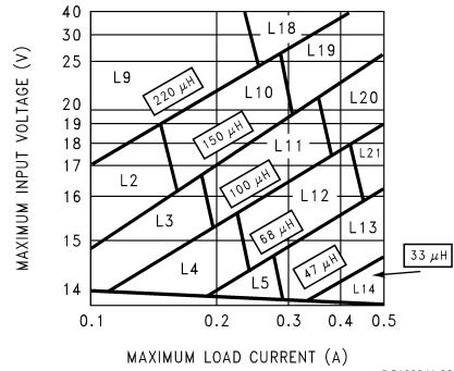
FIGURE 6. LM2674-12
