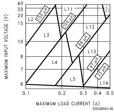
FIGURE 4. LM2674-3.3
