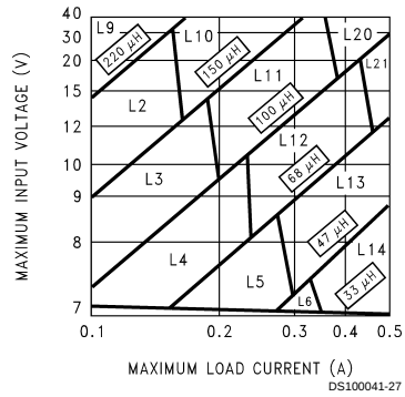
FIGURE 5. LM2674-5.0
