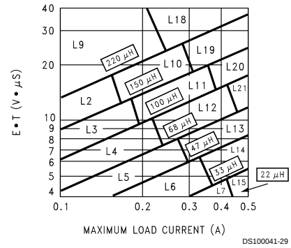
FIGURE 7. LM2674-ADJ
