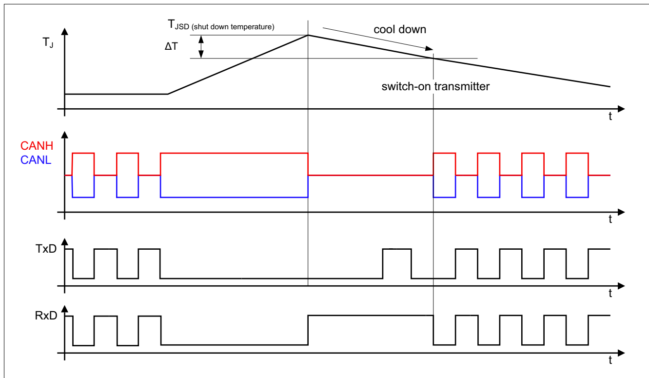
Figure 27 Overtemperature protection
