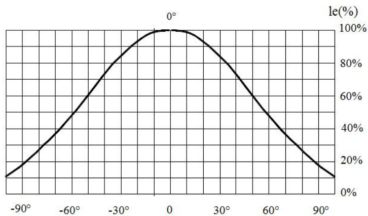
FIG.5 FAR FIELD PATTERN
