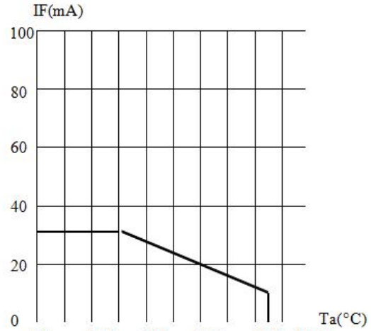
FIG.2 MAXIMUM FORWARD DC CURRENT VS AMBIENT TEMPERATURE ( T_{jmax}=105^{\circ}\text{C} )
