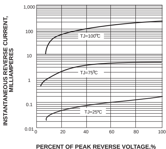
FIG. 4-TYPICAL REVERSE CHARACTERISTICS
