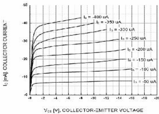
Figure 1. Static Characteristic
