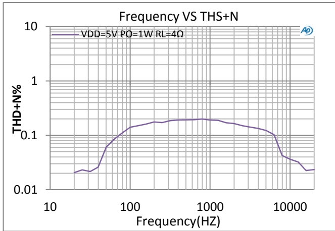
图5: Frequency VS.THD+N
