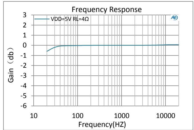
图6: Frequency Response
