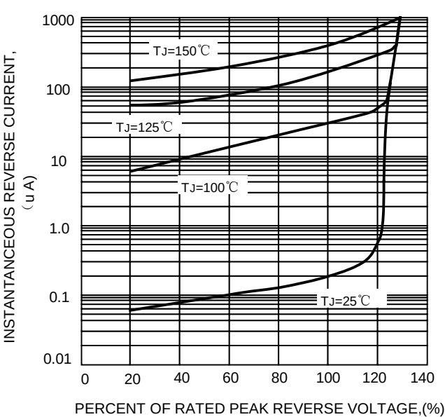
FIG.5-TYPICAL REVERSE CHARACTERISTICS
