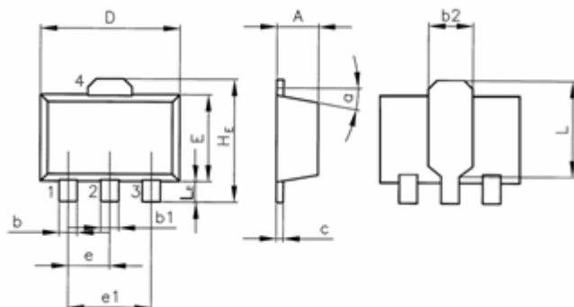
Fig.7 Outline Dimensions
