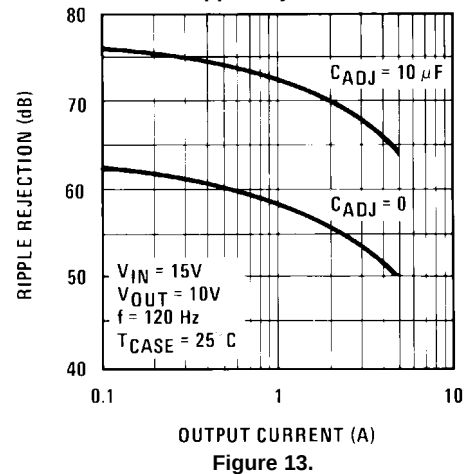
Ripple Rejection
