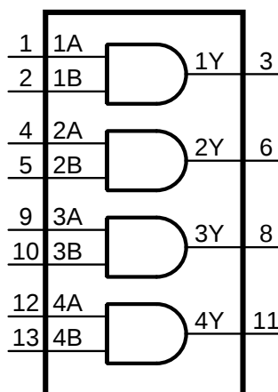
Figure 1. Logic symbol
