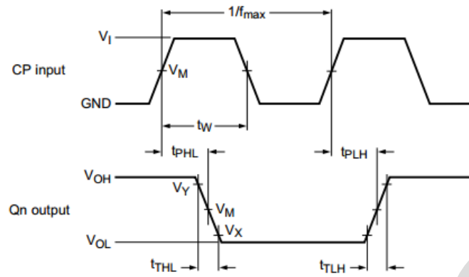
Figure 6. Waveforms showing the clock (CP) to output (Qn) propagation delays, the clock pulse width, the output transition times and the maximum clock frequency
