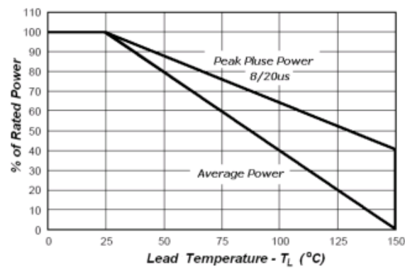
Fig3. Power Derating
