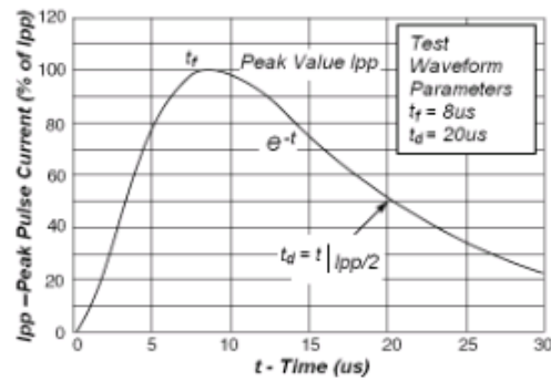
Fig1. Pulse Waveform
