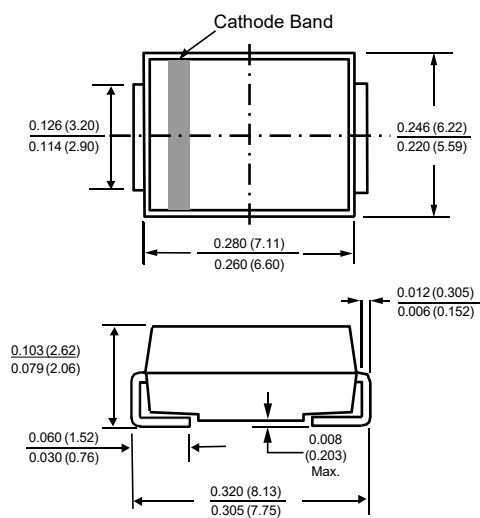
SMC (DO-214AB)
