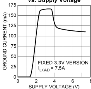
MIC2975x Ground Current vs. Supply Voltage
