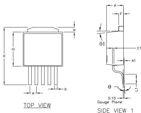
SIDE VIEW 1
