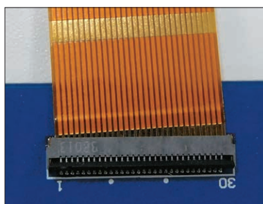
✗ Skewed FPC Insertion
