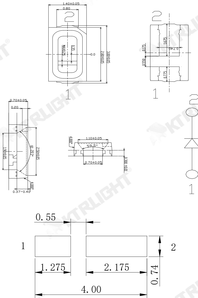
推荐焊盘式样(Recommended Soldering Patter)
