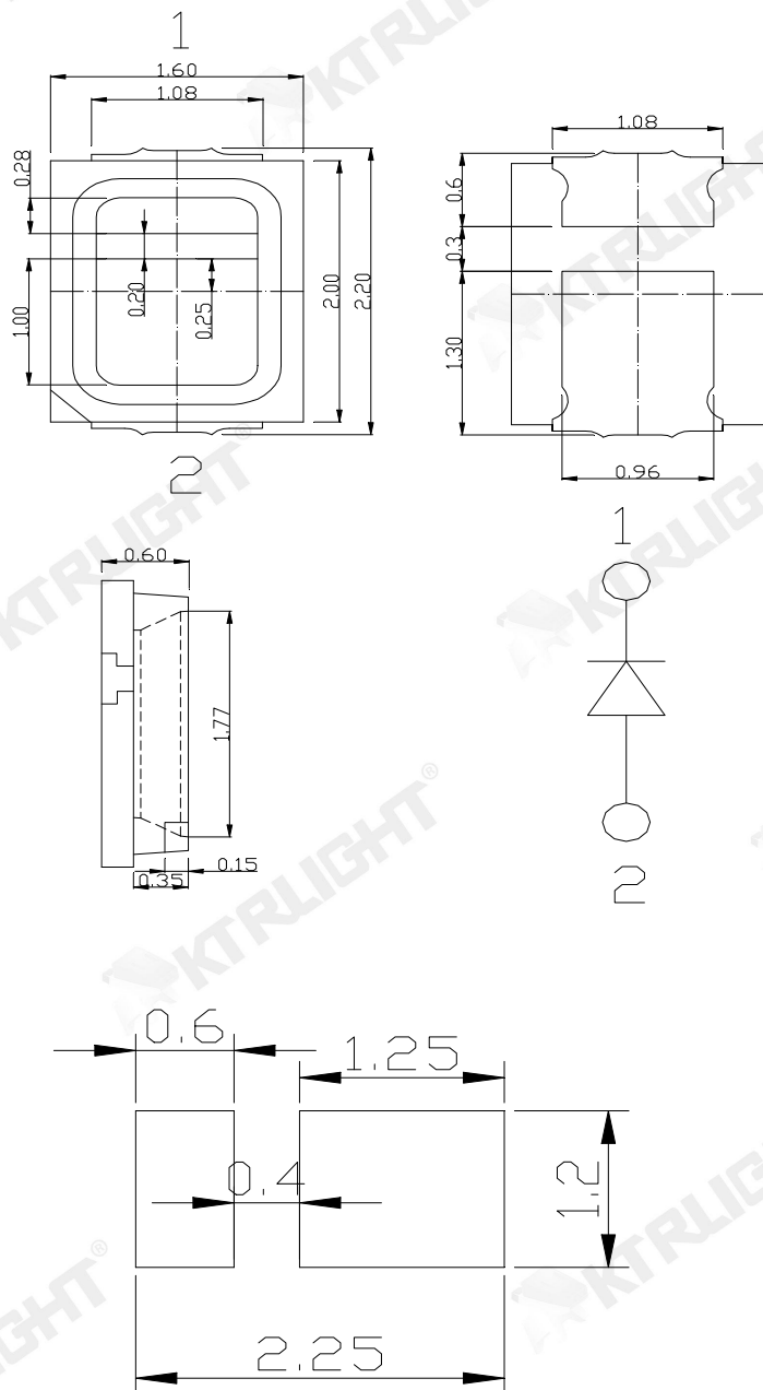
推荐焊盘式样 (Recommended Soldering Patter)
