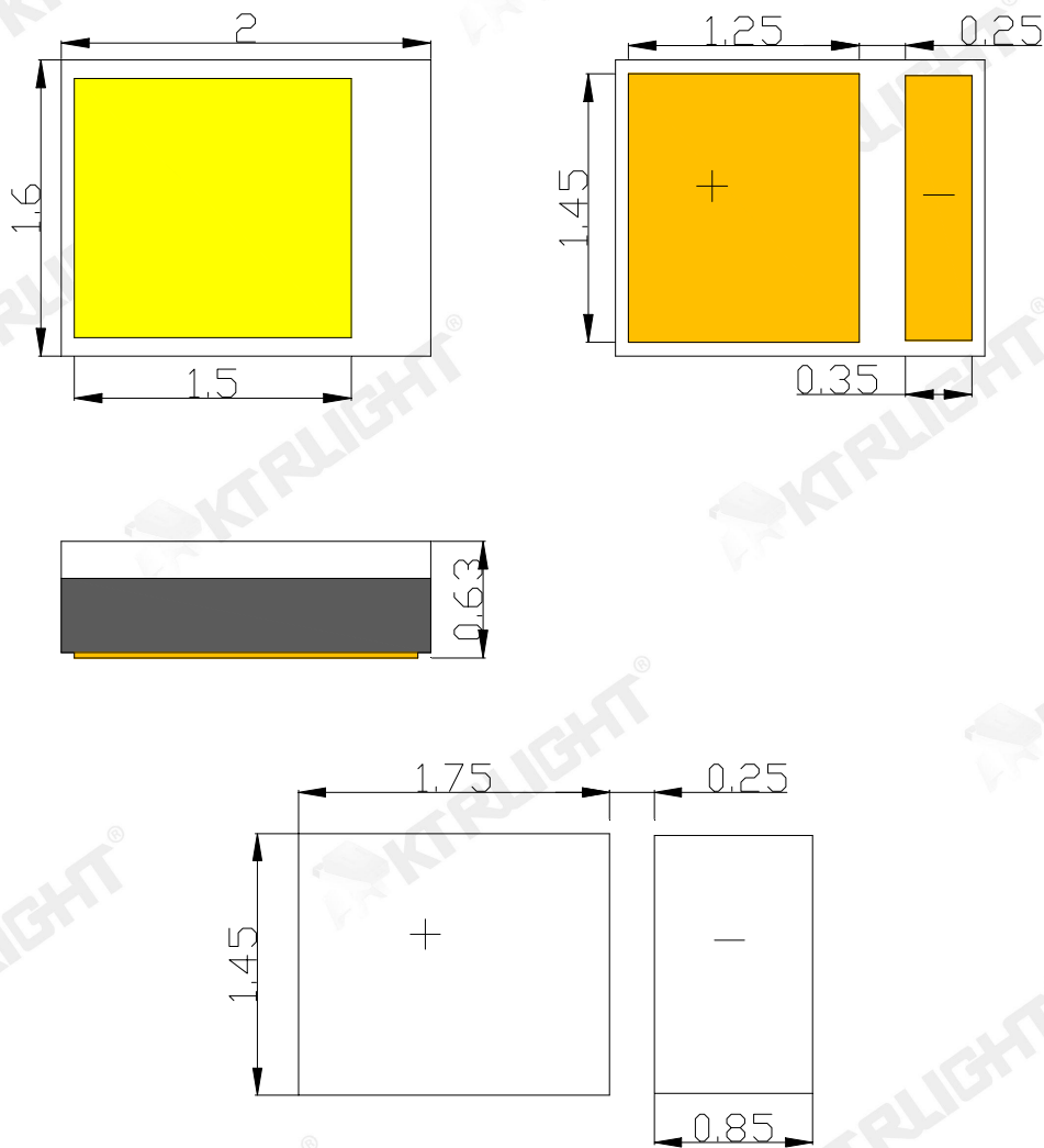
推荐焊盘式样(Recommended Soldering Patter)
