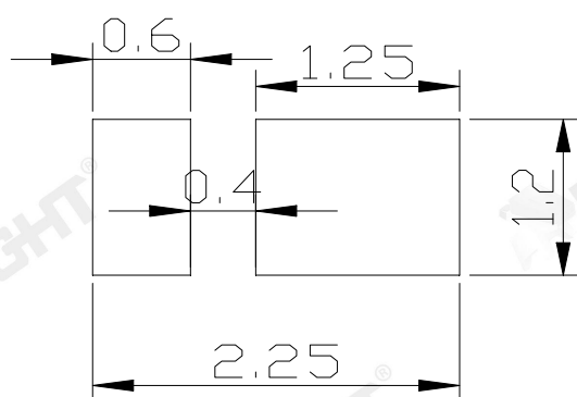
推荐焊盘式样 (Recommended Soldering Patter)
