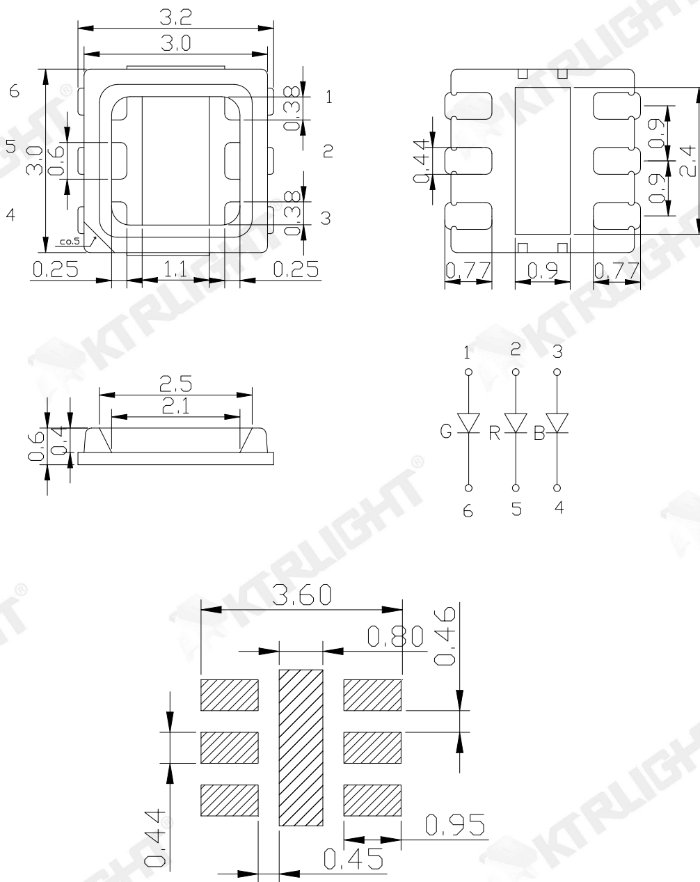
推荐焊盘式样 (Recommended Soldering Patter)
