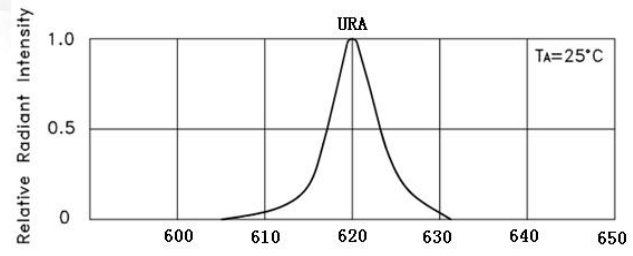
wavelength \lambda (nm) RELATIVE INTENSITY Vs. WAVELENGTH
