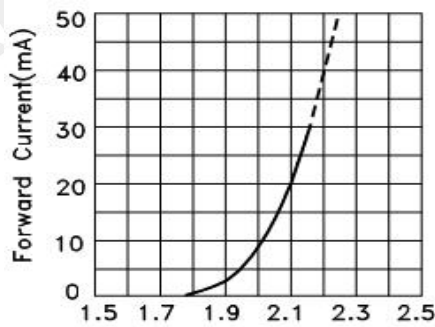
Forward Voltage(V) FORWARD CURRENT Vs. FORWARD VOLTAGE
