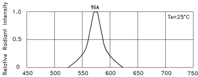
wavelength \lambda (nm) RELATIVE INTENSITY Vs. WAVELENGTH
